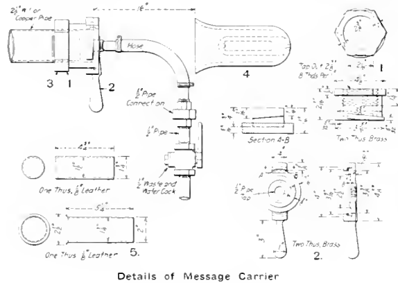
Details of Message Carrier
